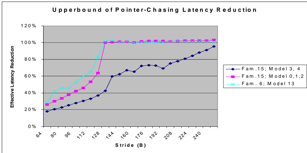
Figure 6-1 Effective Latency Reduction as a Function of Access Stride
