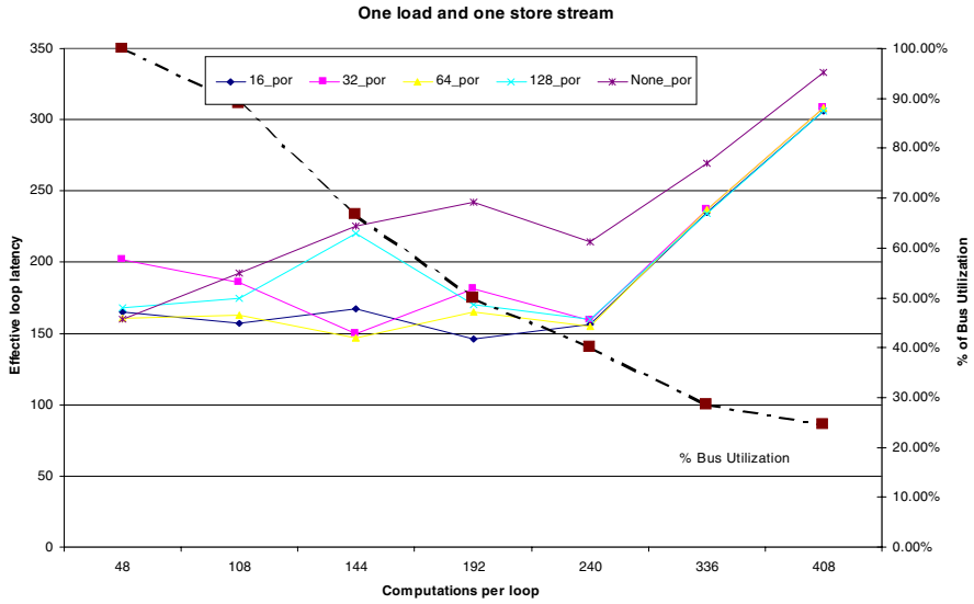
Figure 6-5 Memory Access Latency and Execution With Prefetch
