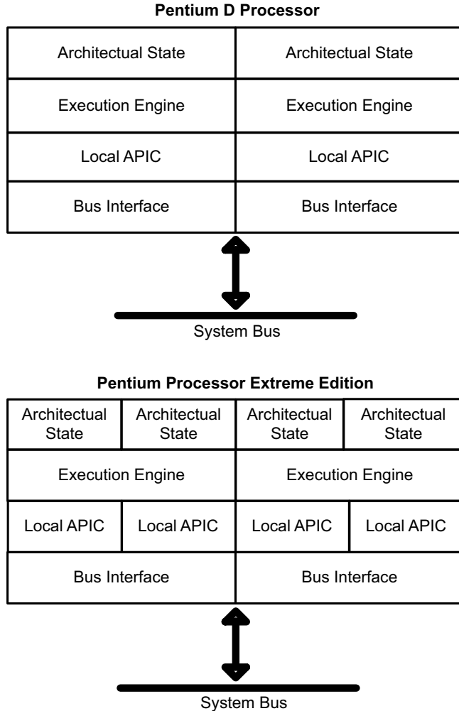
Figure 1-7 Pentium D Processor and Pentium Processor Extreme Edition
