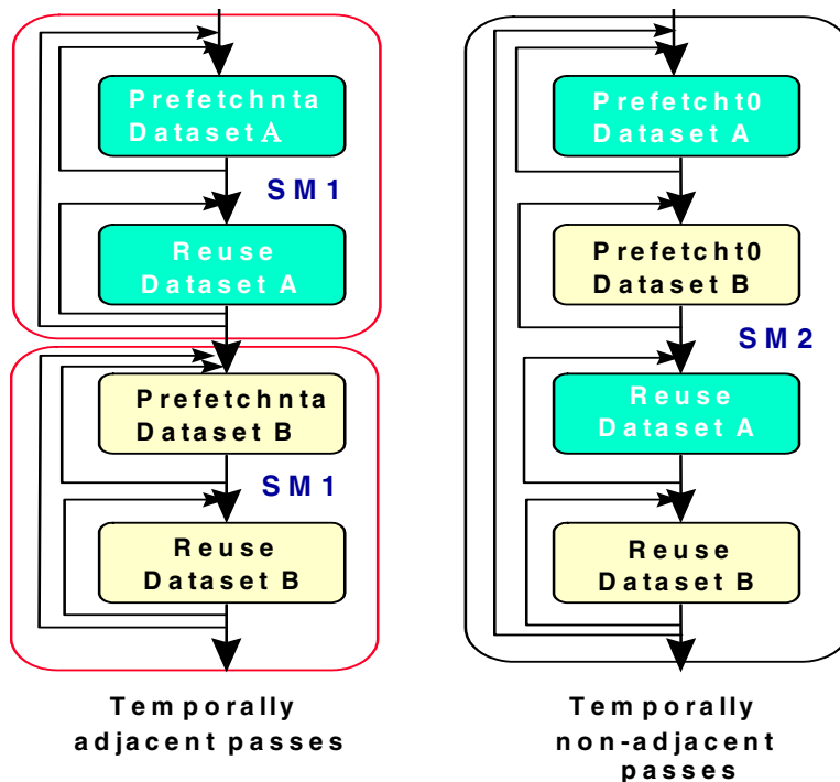
Figure 6-7 Examples of Prefetch and Strip-mining for Temporally Adjacent and Non-Adjacent Passes Loops
