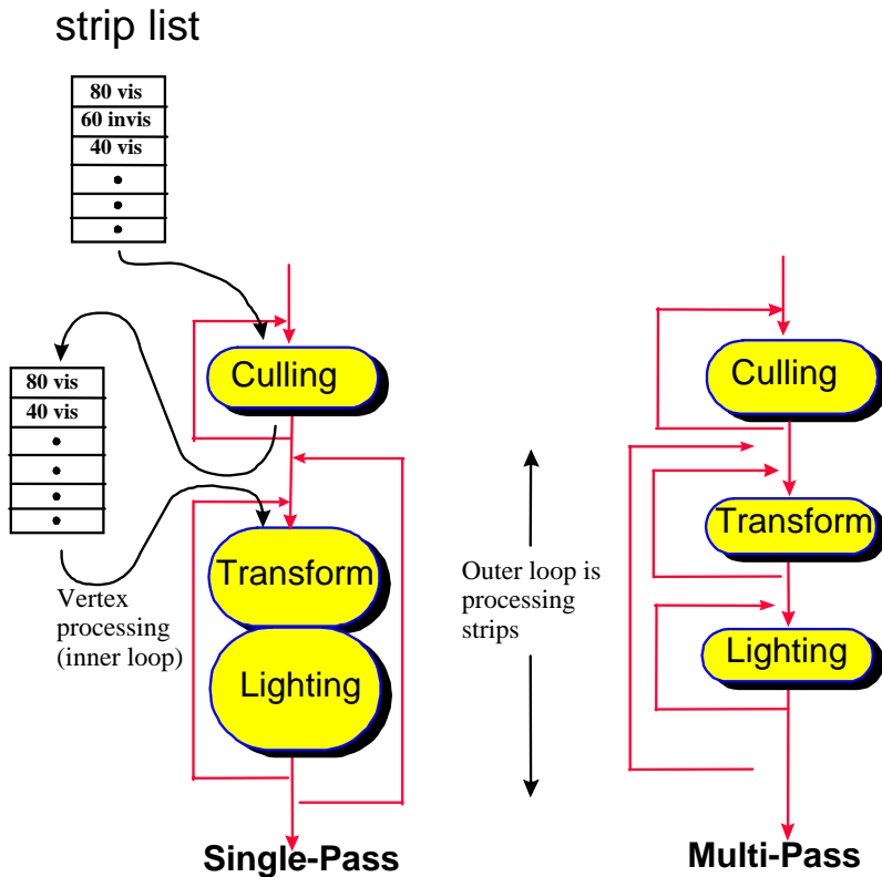
Figure 6-8 Single-Pass Vs. Multi-Pass 3D Geometry Engines
